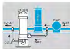
Illustration of Model 300pw Feeder
